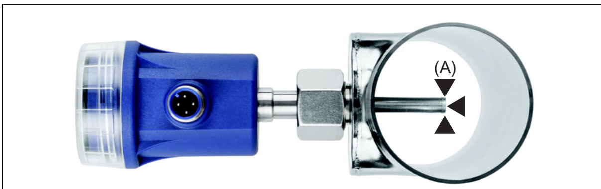
(A) Sensorspitze
