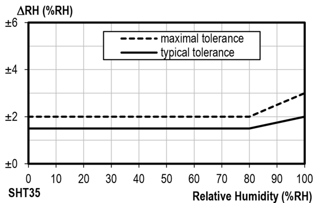
Tolerance of RH at 25°C
