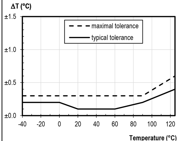
Temperature accuracy
