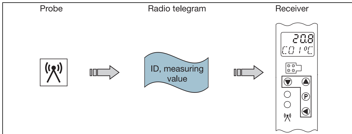
Figure 7: The telegrams of a probe reach the receiver without collisions.
