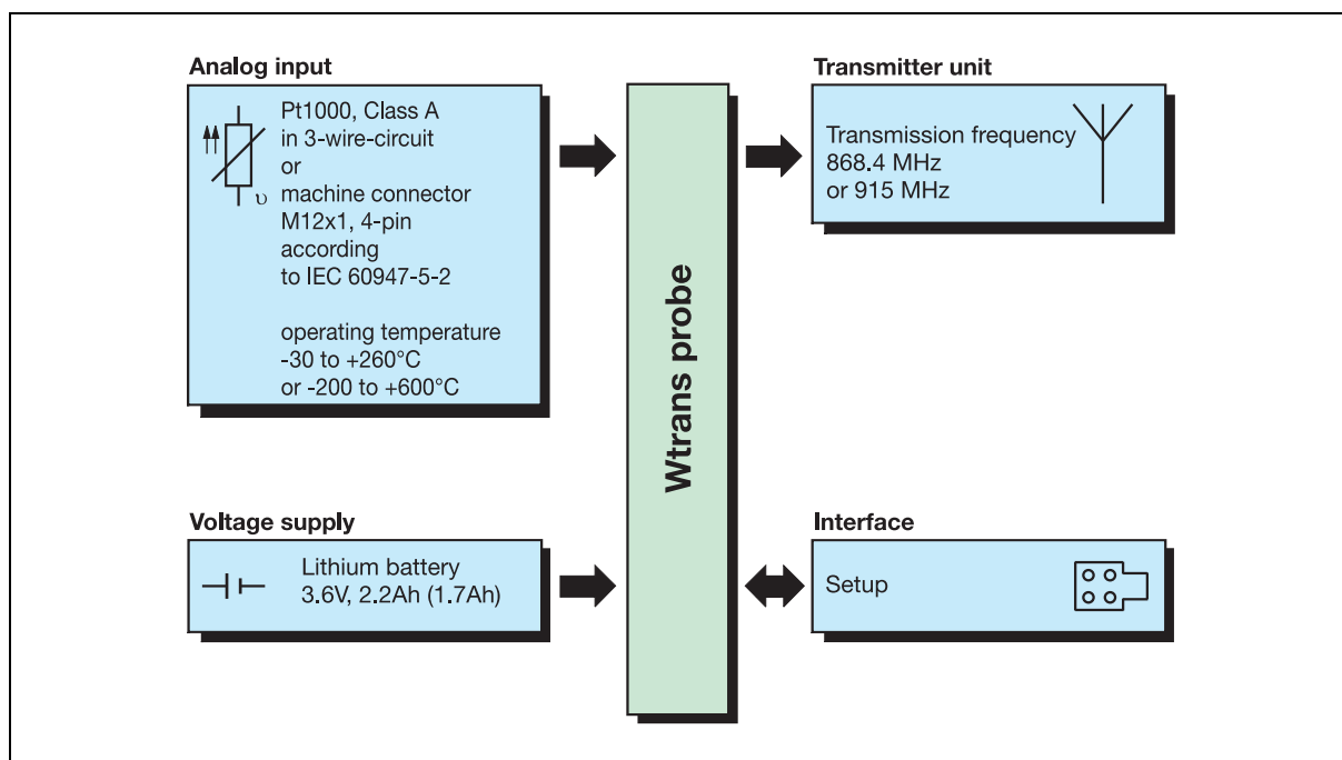
Figure 1: Block diagram of the probe
