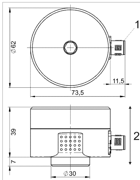
Fig. 3: Housing with M12 connector
