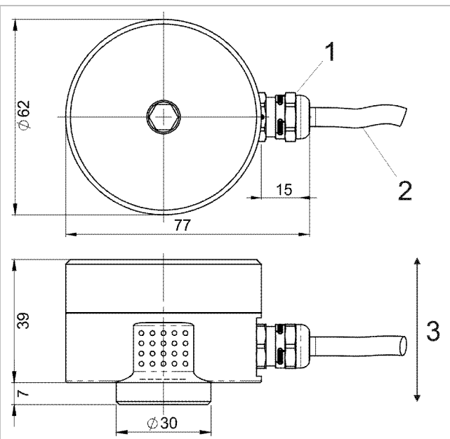
Fig. 4: Housing with integrated cable
