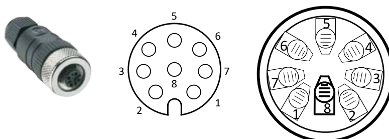
M12 Connector
