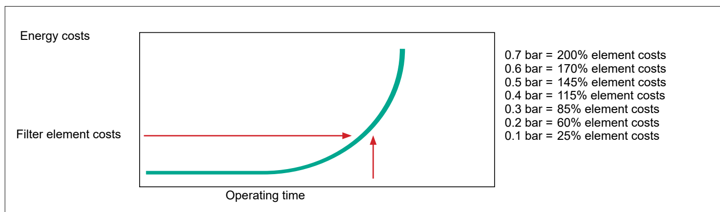
Fig.: Typical differential pressure process, energy costs in relation to filter element costs
