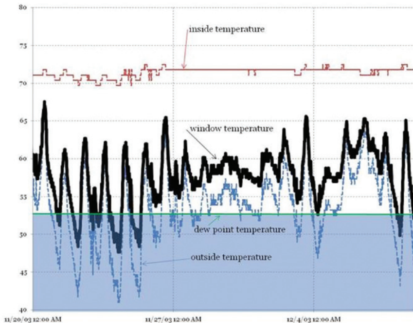
Figure 9: Moisture Investigation
