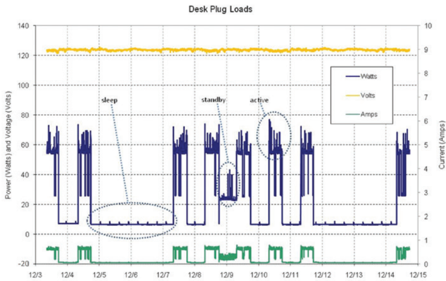
Figure 5: Variation of Desktop Computer Plug Load
