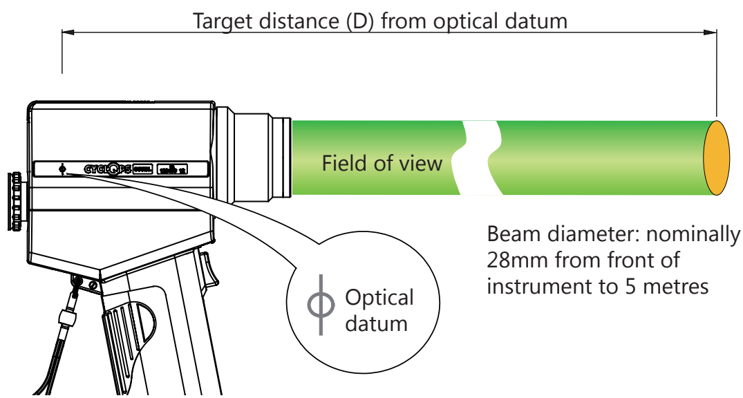
Fig. 6-2 Cyclops 055L thermometer field of view
