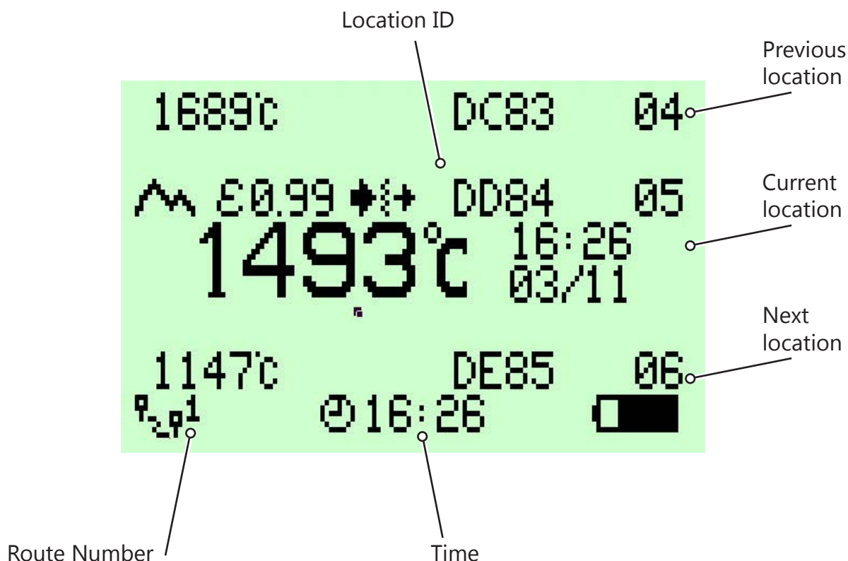
Fig. 7-7 Typical Route Mode display
