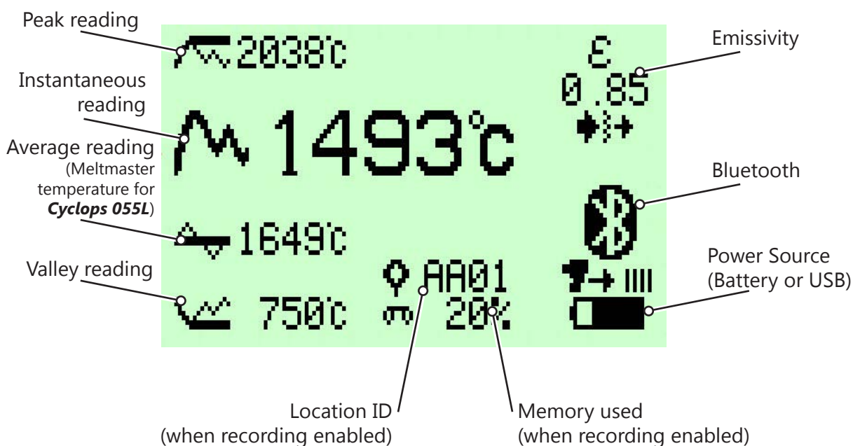
Fig. 7-1 Typical Measure Mode display
