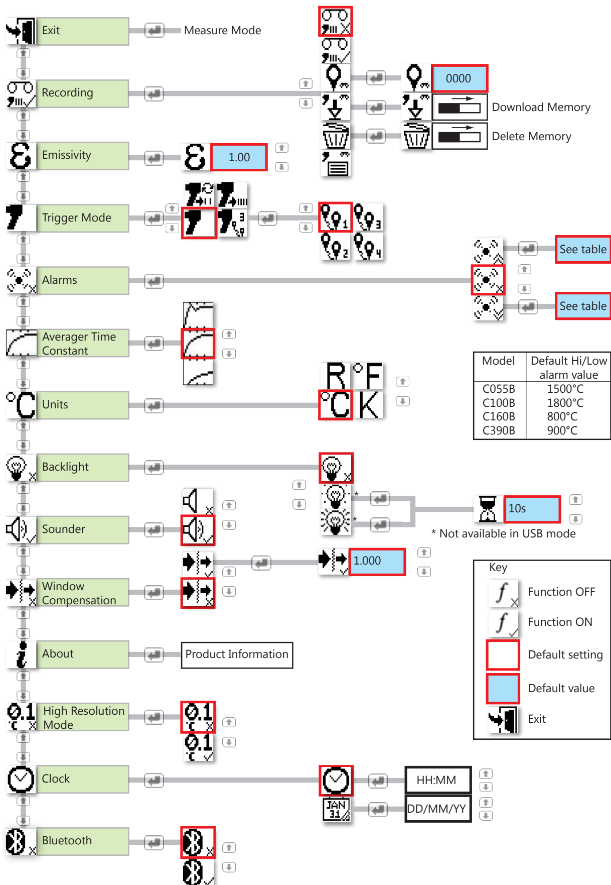
Fig. 7-5 Cyclops menu structure
