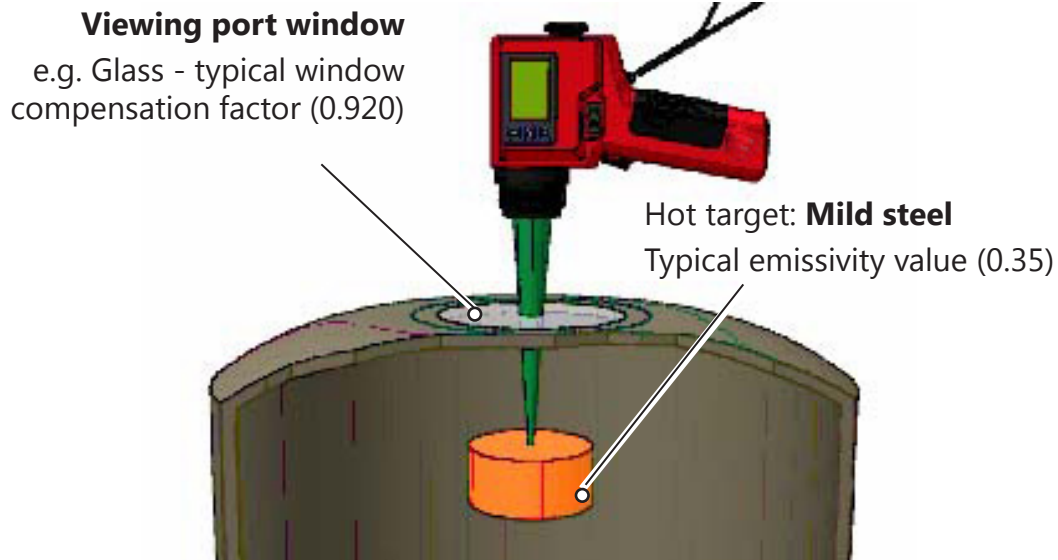
Fig. 9-1 Typical complex temperature measurement application
